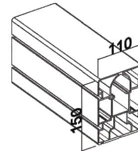
THICK RAIL
