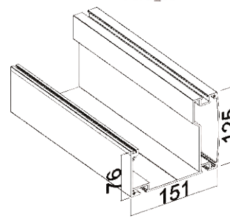
GUTTER
