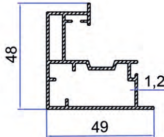
DİKME PROFİLİ SEWING PROFILE 2877 0.736 kg/m
