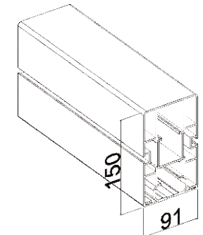
MIDDLE RAIL
